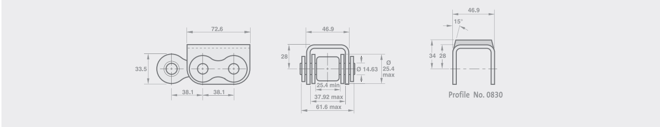
1.500英寸节距简单链条轮廓外形 1.500" pitch simple chain profiles
