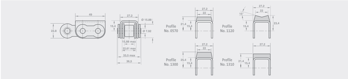
1.000英寸节距简单链条轮廓外形 1.000" pitch simple chain profiles
