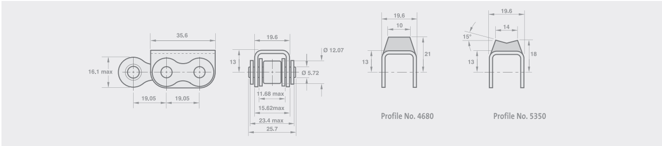
0.750英寸节距简单链条轮廓外形 0.750" pitch simple chain profiles
